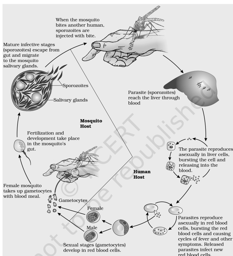
Fig. 7.1 - Stages in the life cycle of Plasmodium .
