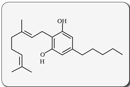
Fig. 7.9 - Skeletal structure of cannabinoid molecule. The plate is a skeletal formula carrying only atom and group symbols (OH, O and H) and no descriptive labels.
